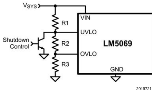
FIGURE 7. Shutdown Control
