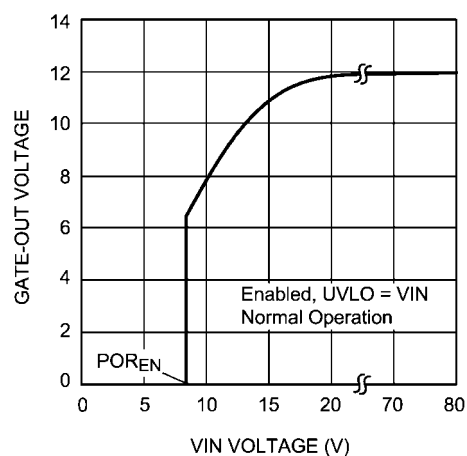
GATE Pin Voltage vs. V_{IN}
