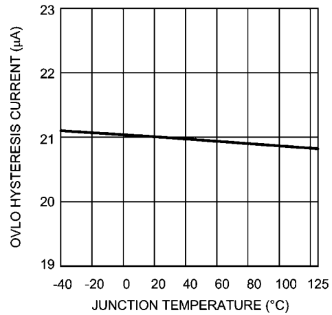
OVLO Hysteresis Current vs. Temperature
