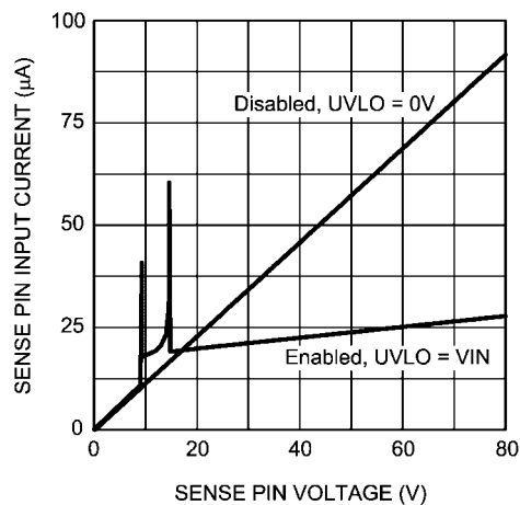
SENSE Pin Input Current
