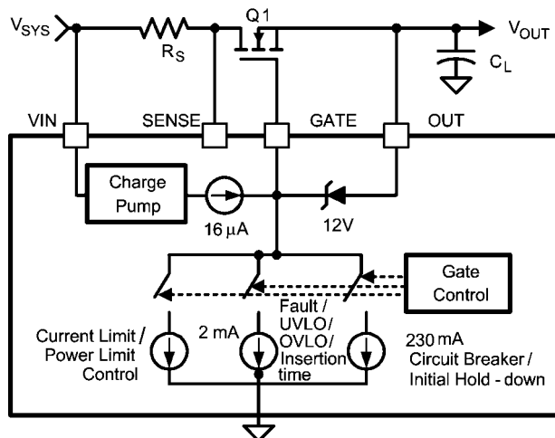
FIGURE 4. Gate Control
